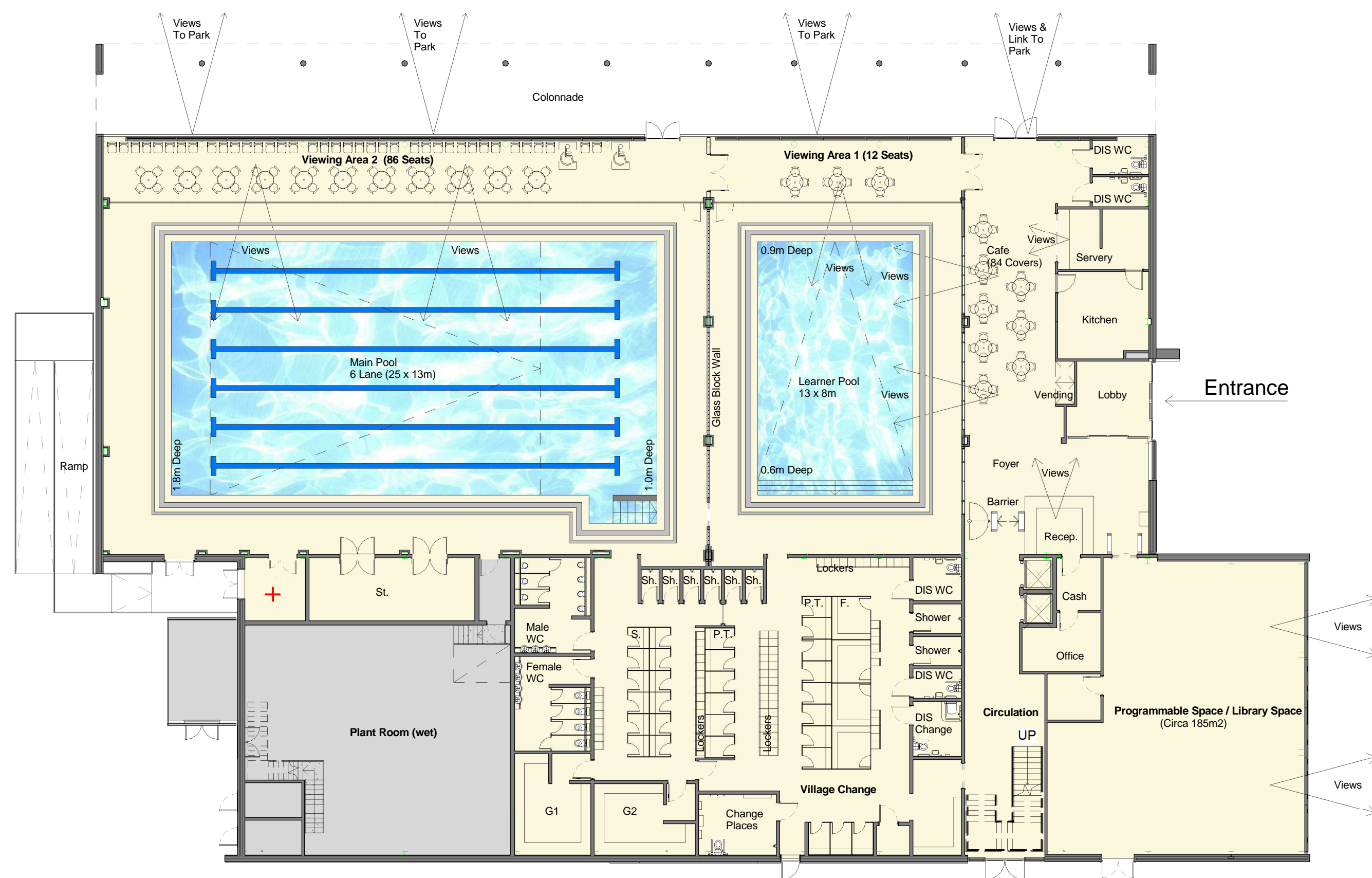
Level 1 - GA Colour - Public Consultation 1 : 200
