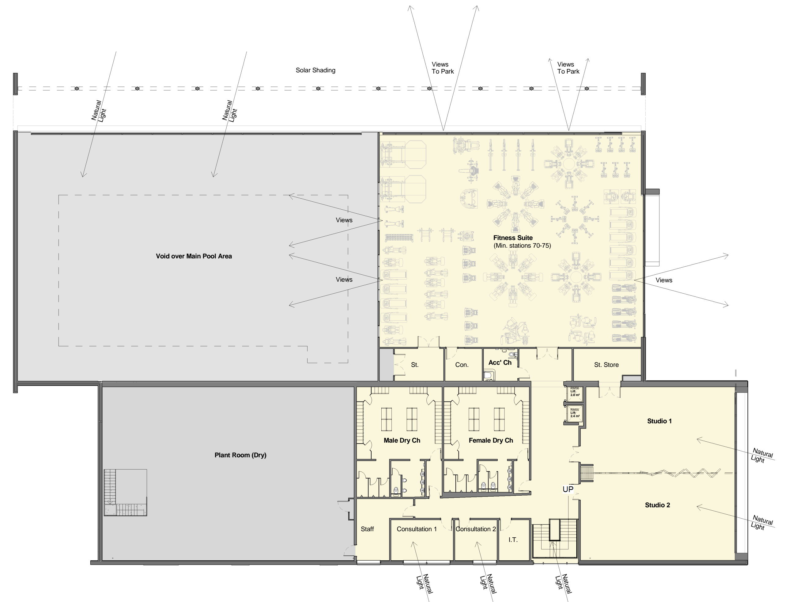
Level 2 - GA Colour - Public Consultation 1 : 200
