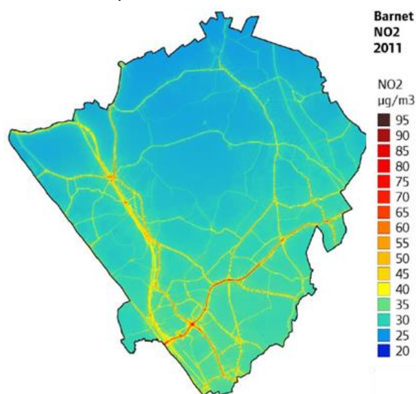
Figure 3-15: Annual Mean Concentrations of NO2 in Barnet, 2011
